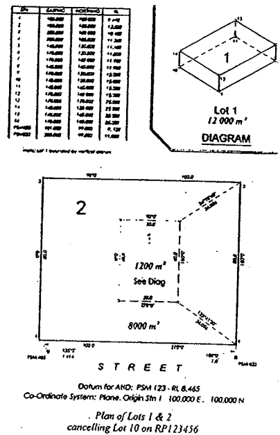
Figure 25.2: Plan showing a volumetric parcel by co-ordinates
