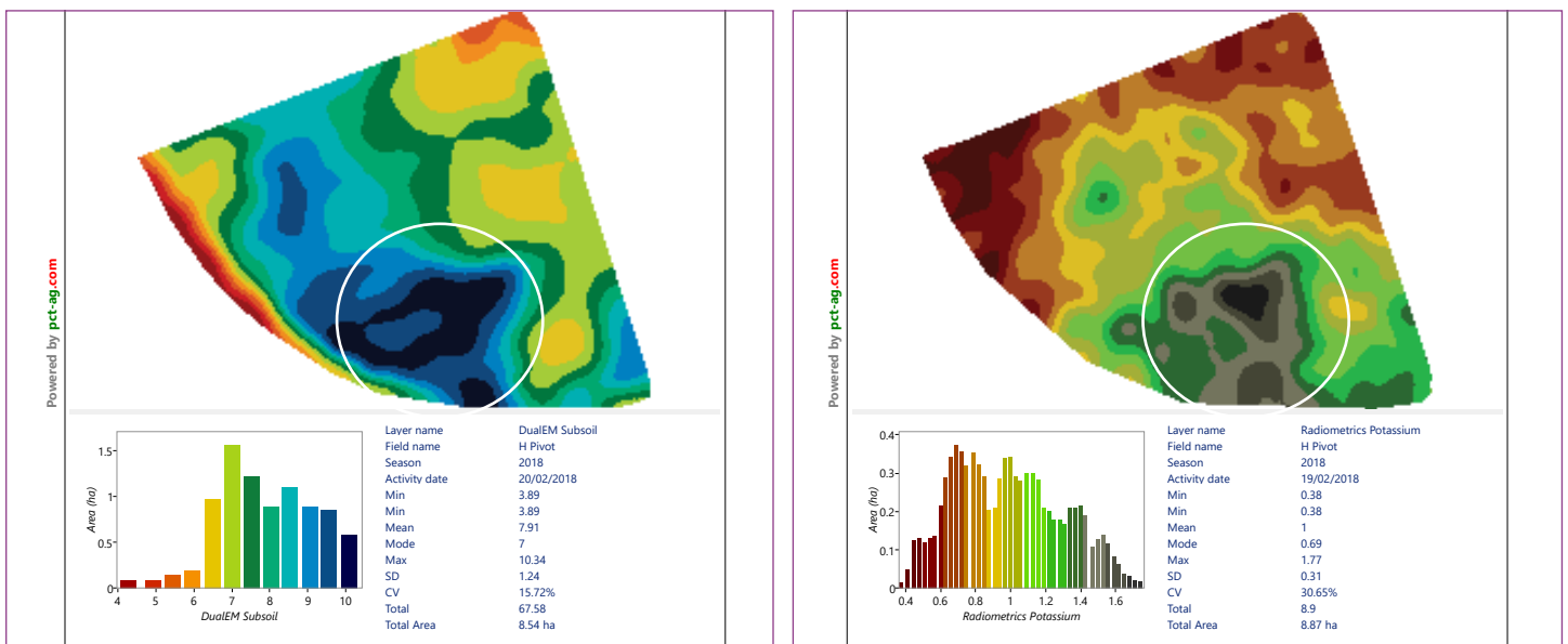
Figure 4. Subsurface EM38 and radiometric data showing differences in the area around Wildeye 2.
