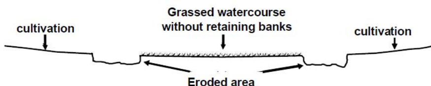
Figure 4. Waterways without retaining banks are likely to erode on either side of the grass strip
