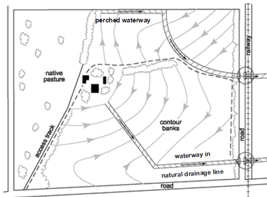
Figure 1. A contour bank and waterway layout for erosion control in a cultivated paddock
