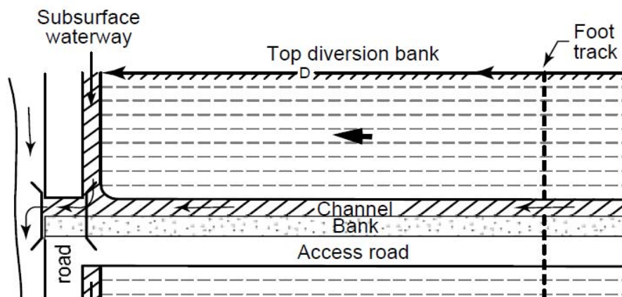
Figure 7. Row crops draining into a subsurface waterway
